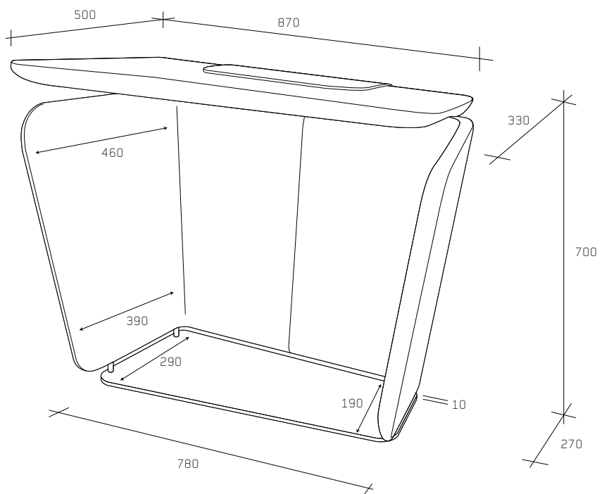
Type 003.04 | With assymetric sides
