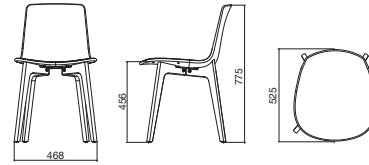
Silla respaldo standard Chair standard back
